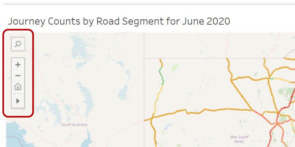
Figure 7: Navigation Bar
