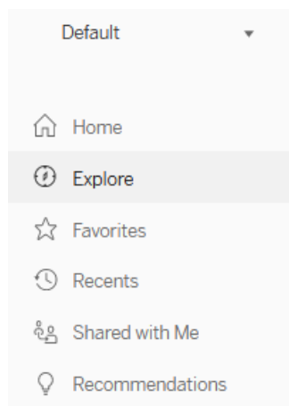
Figure 2: Navigation Menu
