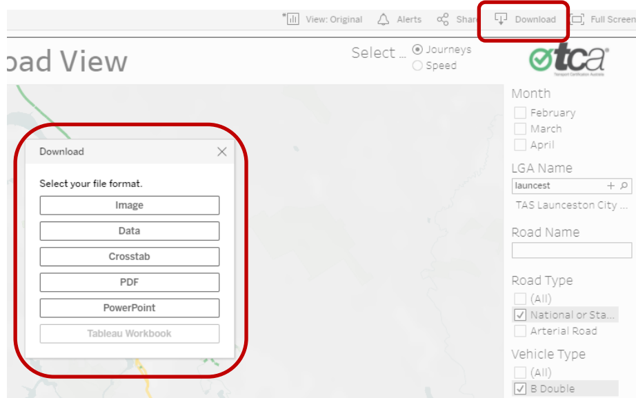
Figure 11: Exporting Data
