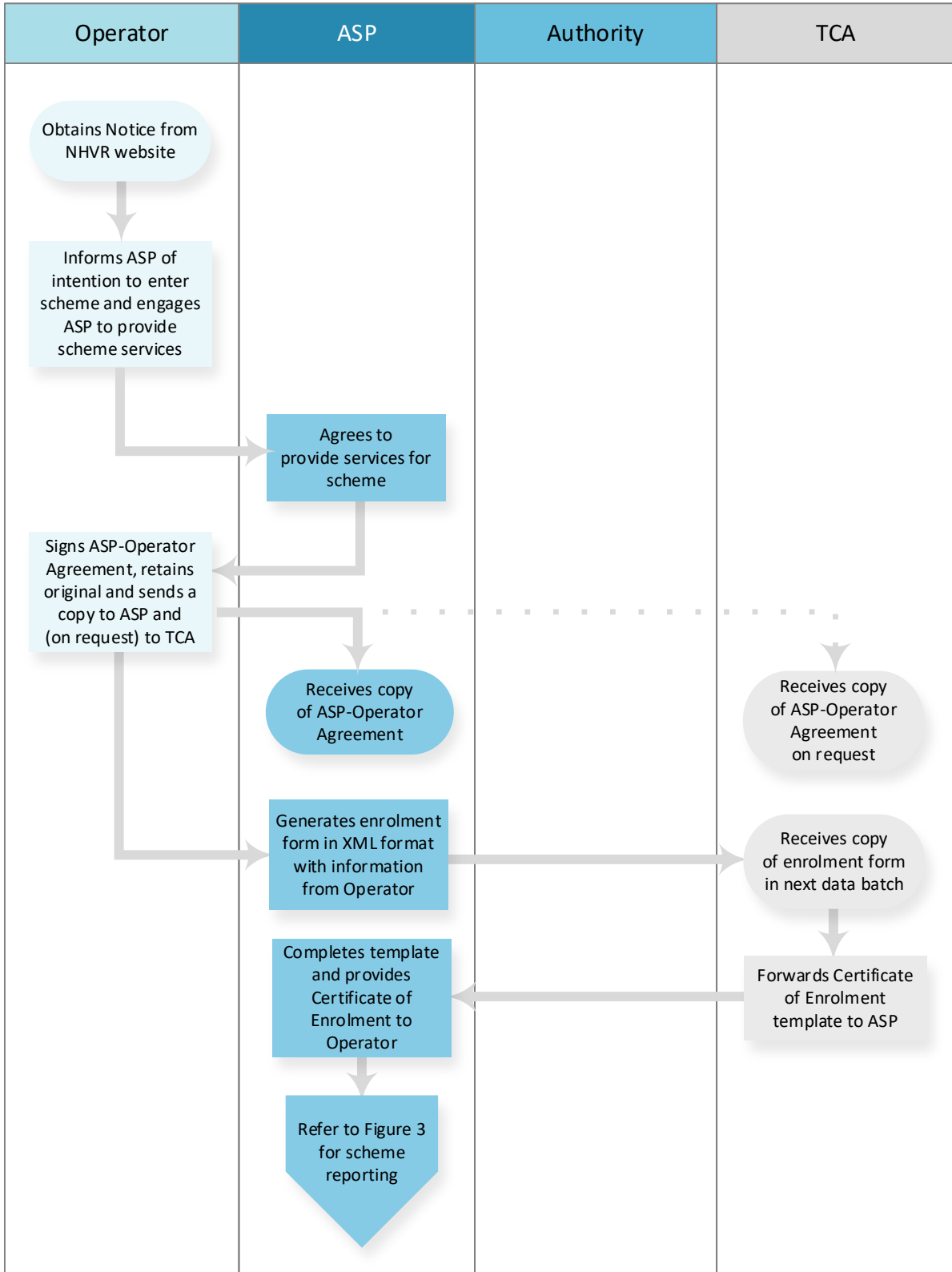
Figure 2: Pre-Enrolment Process
